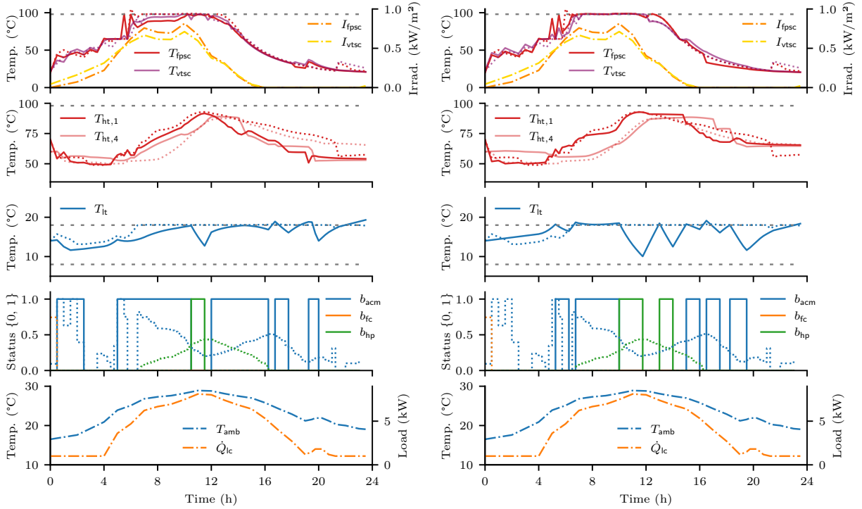
Fig. 6. Comparison of the system trajectories computed at the first iteration of the algorithm (left) and at iteration 23 (right), which is the best determined solution in terms of the objective. The state bounds are expressed in the plots by horizontal dashed gray lines. The dotted lines are the trajectories of the relaxed solutions (the initial guess) and the dash-dotted lines correspond to the ambient conditions. Specifically, the solar irradiation on the vacuum tube solar collectors I_{vtsc} and on the flat plate solar collectors I_{fpvc} , the ambient temperature T_{amb} , and the cooling load profile \dot{Q}_{lc} .
