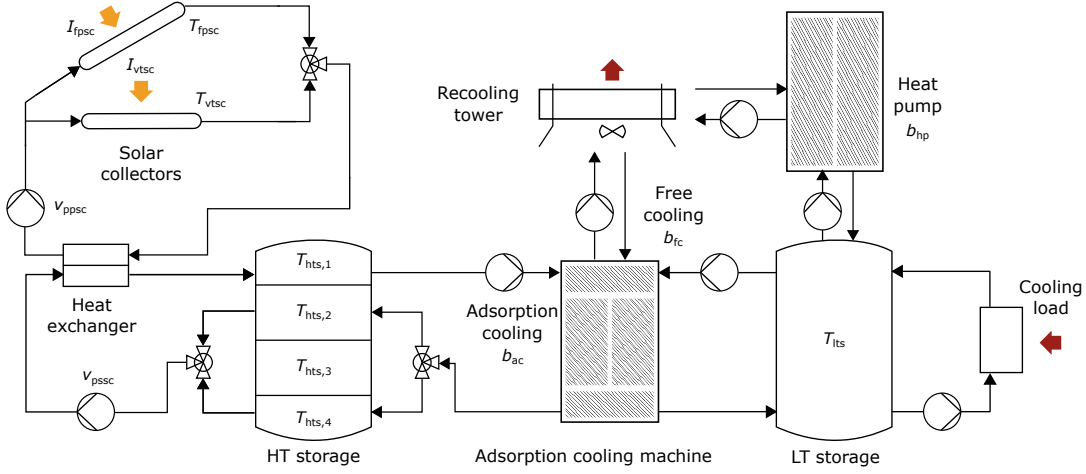
Fig. 3. Schematic of the energy system considered. A detailed explanation of the system can be found in [13].
