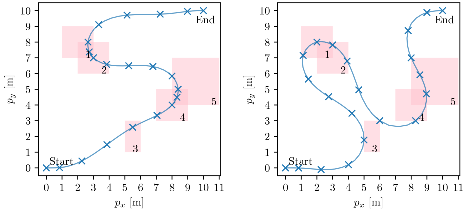
FIGURE 5 | Locally optimal UGV position trajectories for MINLP (left) and MPVC (right) for (44a).
