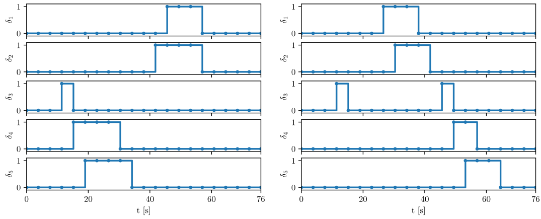
FIGURE 6 | Locally optimal trajectories of indicator variables for MINLP (left) and MPVC (right) for (44a).
