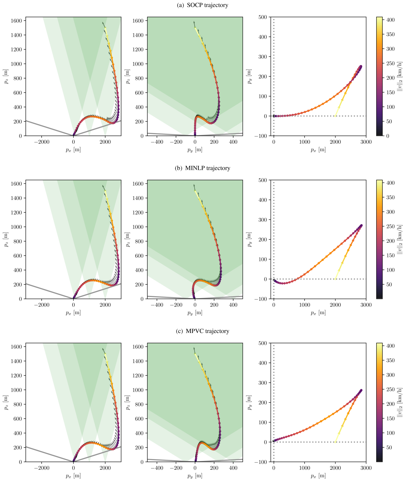
FIGURE 7 | Spacecraft trajectories for SOCP (top), MINLP (50) (middle), and MPVC (51) (bottom). For each, the three plots show the trajectories of the position projected onto the xz , yz , and xy planes, respectively. The color used to depict the trajectory shows the Euclidean norm of the lander's velocity. The direction of the gray arrows represents the pointing angle of the lander in every discretization point, and the length of the arrows represents the Euclidean norm of the thrust. The green areas represent the divert-feasible regions. The gray solid lines at the bottom of the left and middle plots represent the glide-slope constraint. The position is constrained to be above such lines.
