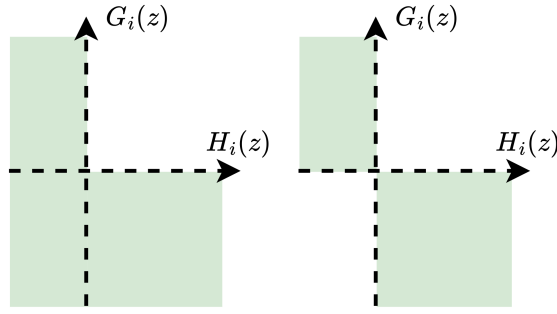
FIGURE 2 | Left: in light green the feasible set of constraint (25) (the indicator variable \delta_i is projected out). Right: in light green, the feasible set of constraint (26). In both plots the dashed lines are part of the feasible set. The MPVC constraints (26) do not correctly represent the logical implication. By considering (27), we obtain two identical feasible sets and a correct representation of the logical implication. However, this introduces unnecessary restrictions for the MINLP formulation.
