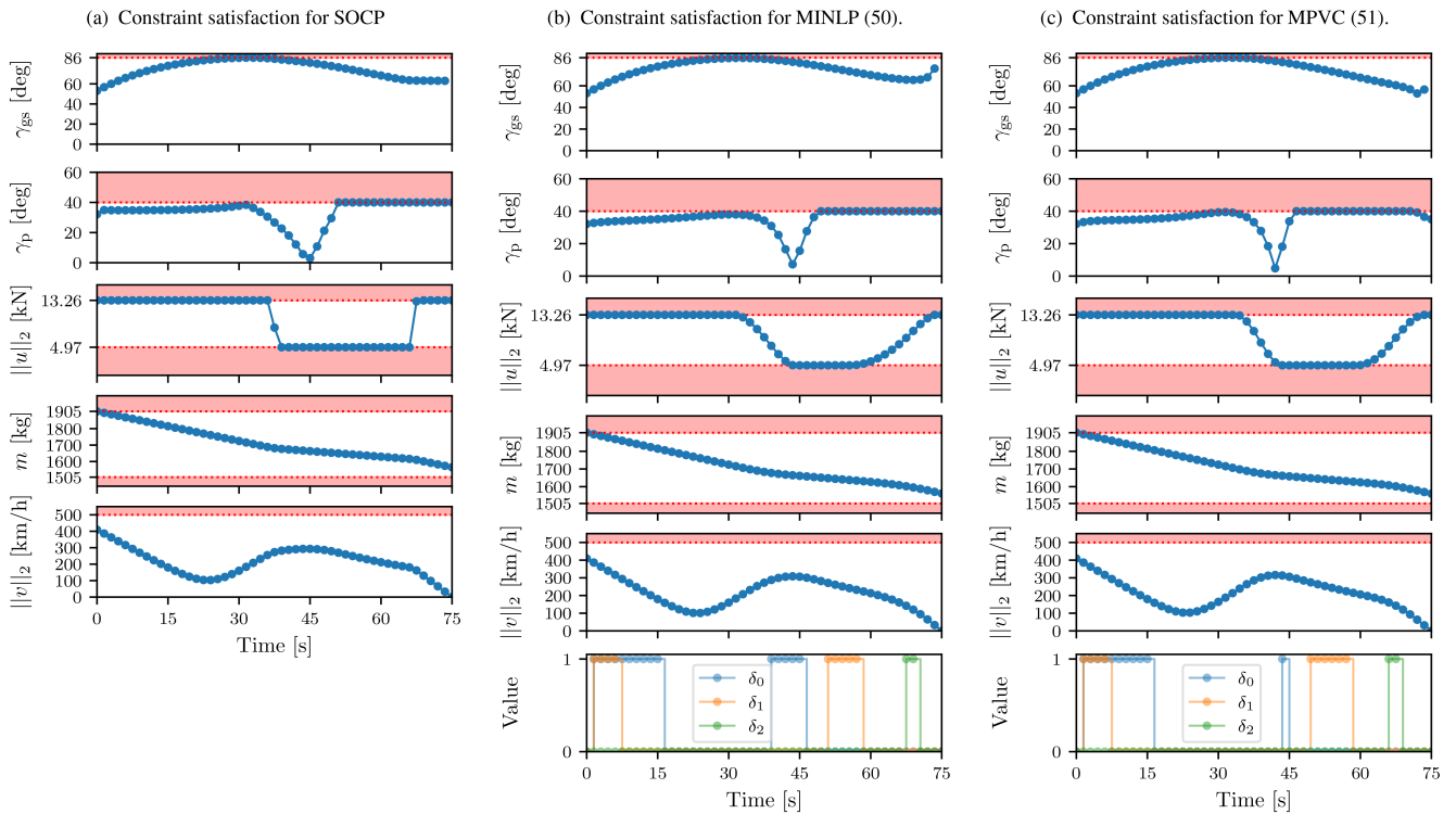
FIGURE 8 | Comparison of constraint satisfaction for the time- and fuel-optimal problem (no polyhedral constraints) SOCP (left), against MINLP (50) (middle), and MPVC (51) (right). From top to bottom, the subplots represent the evolution of glide-slope angle, the evolution of the pointing angle, the Euclidean norm of the thrust, the mass depletion, and the Euclidean norm of the lander's velocity. The bottom subplot in the middle and right plot represents the trajectory of the indicator variables \delta , that is, the membership in divert-feasible regions.
