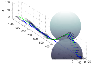
Fig. 9. Obstacle avoidance, 3D trajectory. The dotted curve is the reference trajectory \gamma . The aircraft trajectory is the solid line. The aircraft attitude is represented by the triangles.
