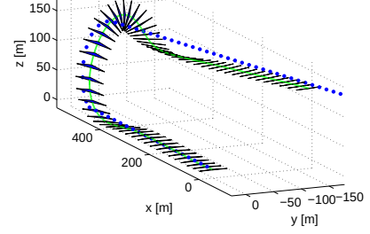
Fig. 4. Flip, 3D trajectory. The dotted curve is the reference trajectory \gamma . The aircraft trajectory is the solid line. The aircraft attitude is represented by the triangles.
