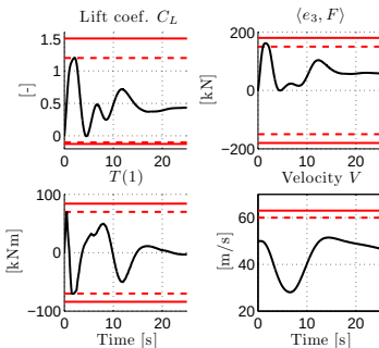
Fig. 10. Obstacle avoidance, flight envelope
