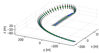
Fig. 6. Aileron failure in a sharp turn, 3D trajectory. The aircraft trajectory is the solid line. The aircraft attitude is represented by the triangles.
