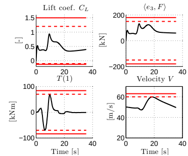
Fig. 7. Ailerons failure in a turn, flight envelope
