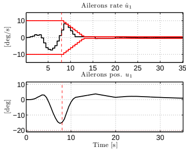
Fig. 8. Ailerons failure in a turn, ailerons rate and position
