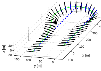
Fig. 2. Fast turn, 3D trajectory. The dotted curve is the reference trajectory \gamma . The aircraft trajectory is the solid line. The aircraft attitude is represented by the triangles.
