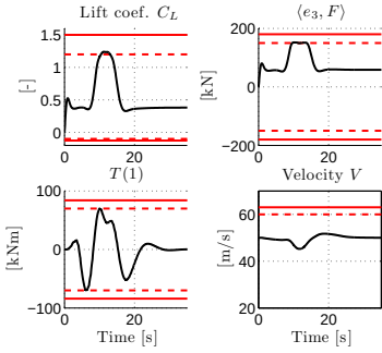
Fig. 3. Fast turn, flight envelope. The dashed lines are the constraints with back-off, the solid lines are the physical constraints.
