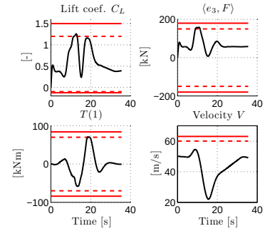
Fig. 5. Flip, flight envelope. The dashed lines are the constraints with back-off, the solid lines are the physical constraints.
